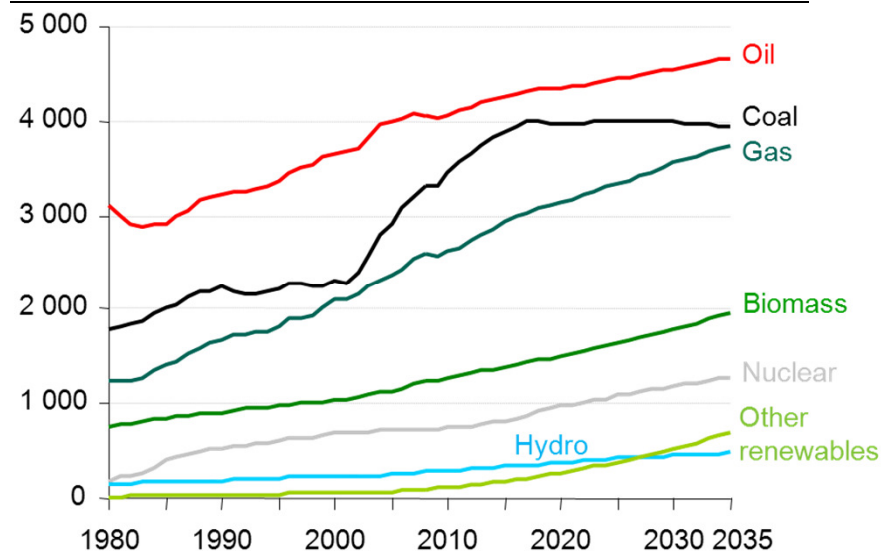
World primary energy demand by fuel in IEA New Policies Scenario In Mtoe
